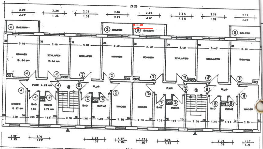
[B] ERDGESCHOSS
